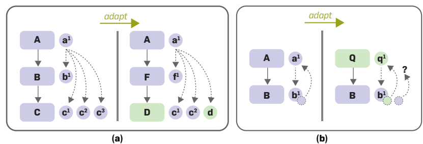
Figure 2. Hot-swapping a single building block (a) and a typical observer pattern relationship (b).
